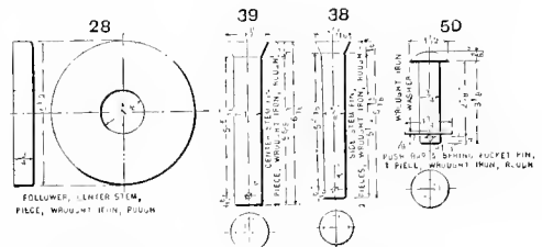
Figs. 1385-1388. Center-stem Follower.
